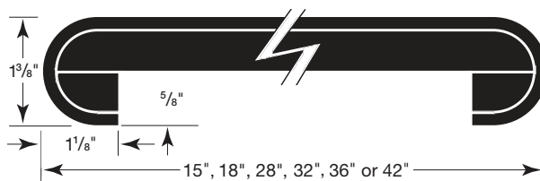
M-DR (Double Roll Bar)
