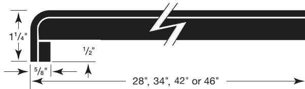
L-SR (Single Roll Bar)
