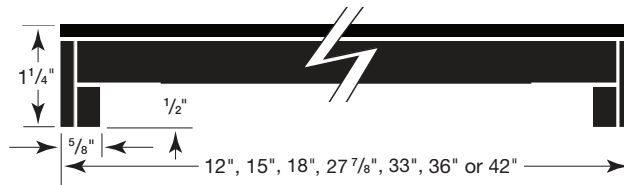
V-DR (Double Sided Bar)
