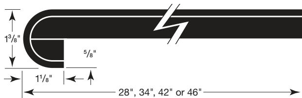
M-SR (Single Roll Bar)
